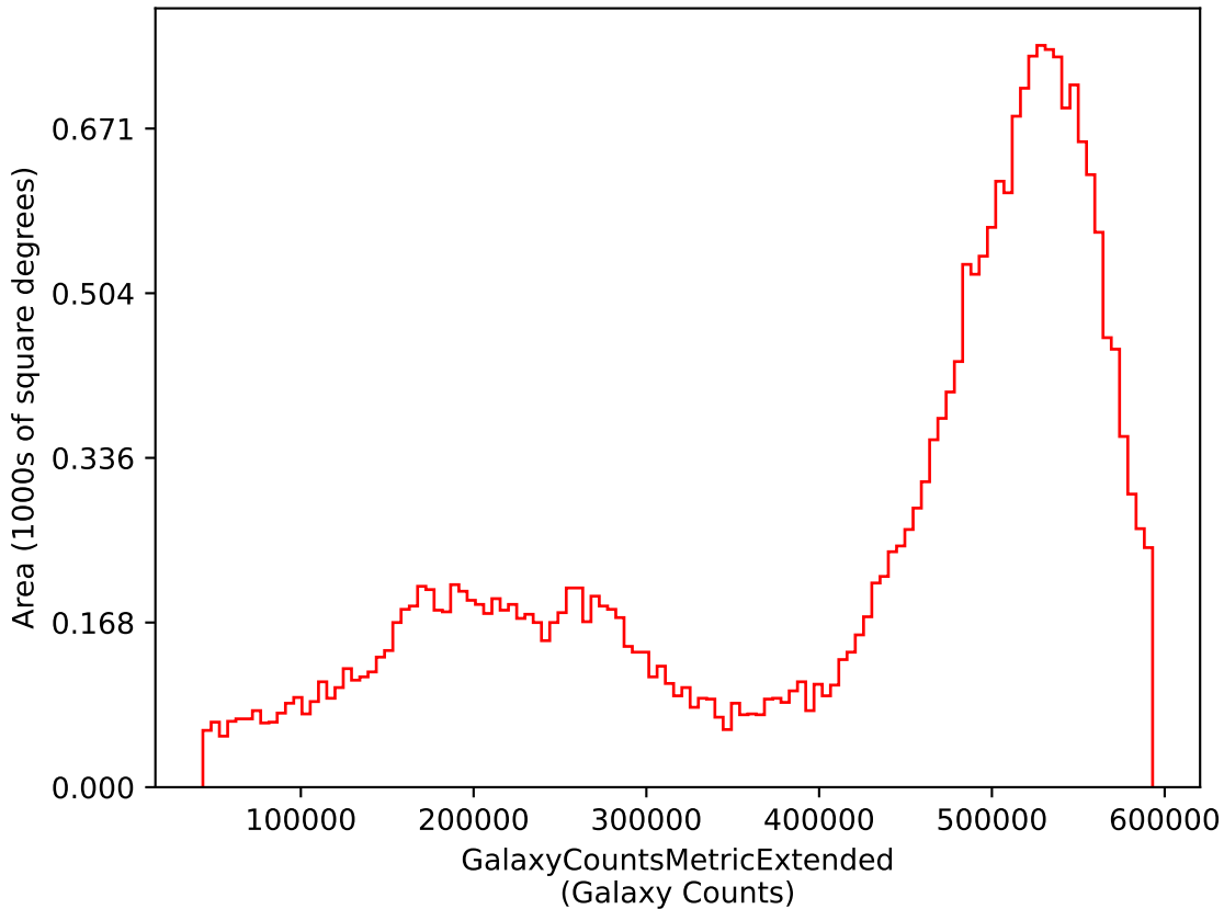
reweight_bulge_v3.3_10yrs i: GalaxyCountsMetricExtended
