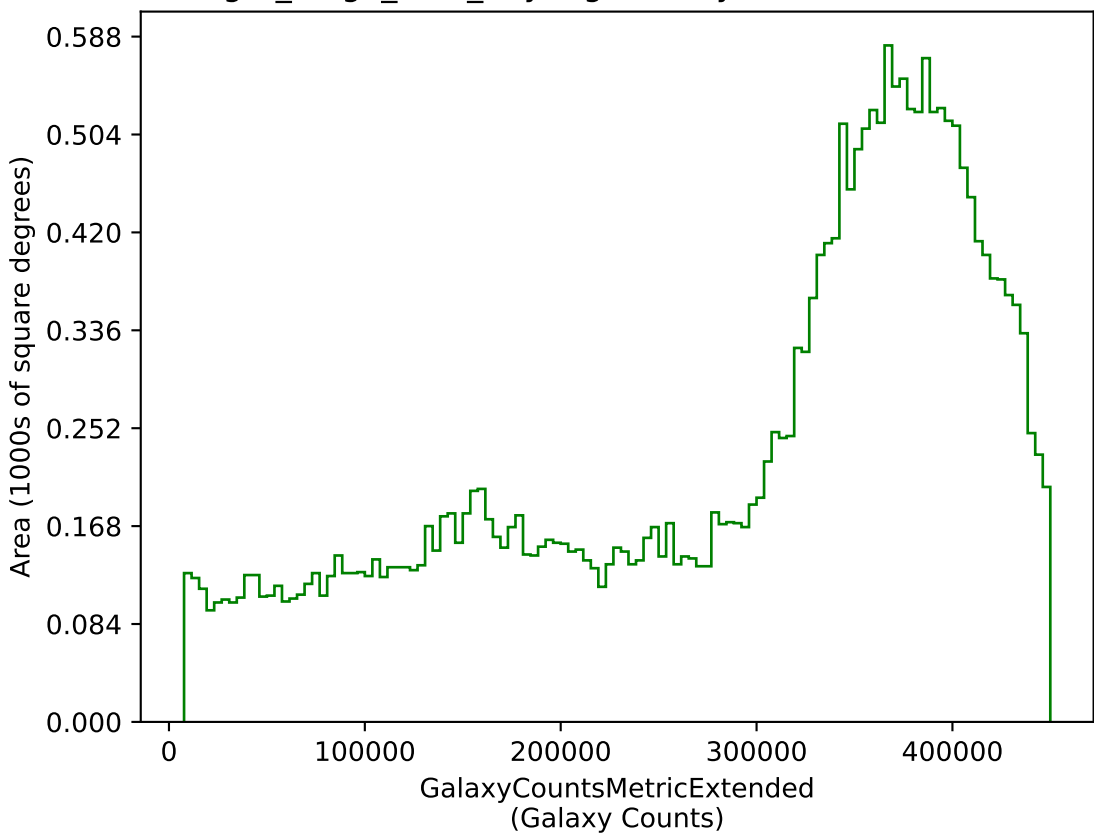
reweight_bulge_v3.3_10yrs g: GalaxyCountsMetricExtended
