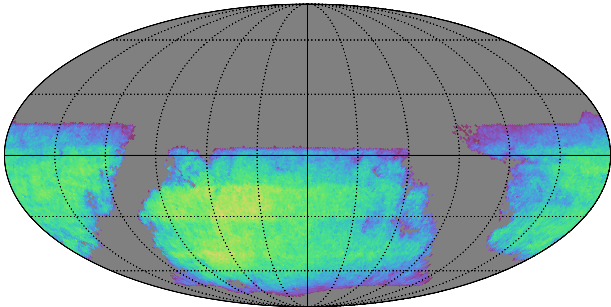
reweight_bulge_v3.3_10yrs i band non-DD year 9: ExgalM5WithCuts
