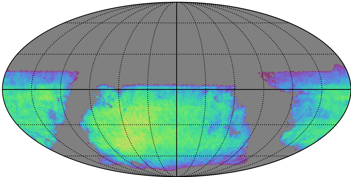
reweight_bulge_v3.3_10yrs i band non-DD year 8: ExgalM5WithCuts
