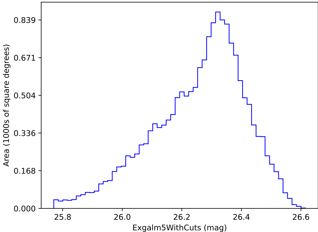
reweight_bulge_v3.3_10yrs i band non-DD year 8: ExgalM5WithCuts
