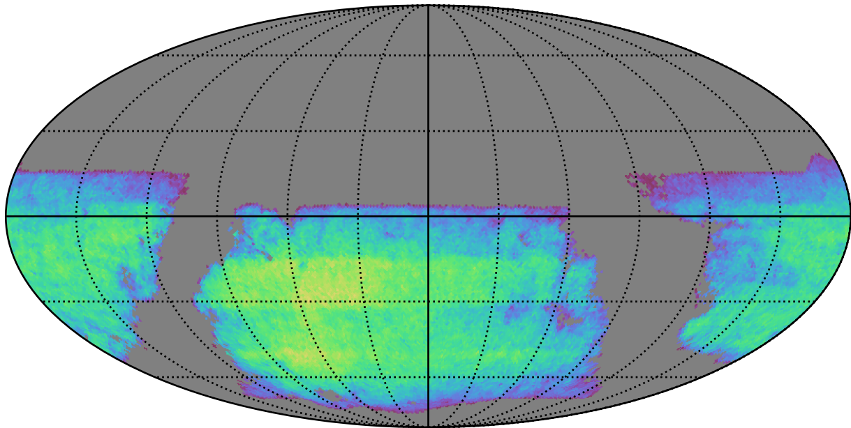
reweight_bulge_v3.3_10yrs i band non-DD year 7: ExgalM5WithCuts
