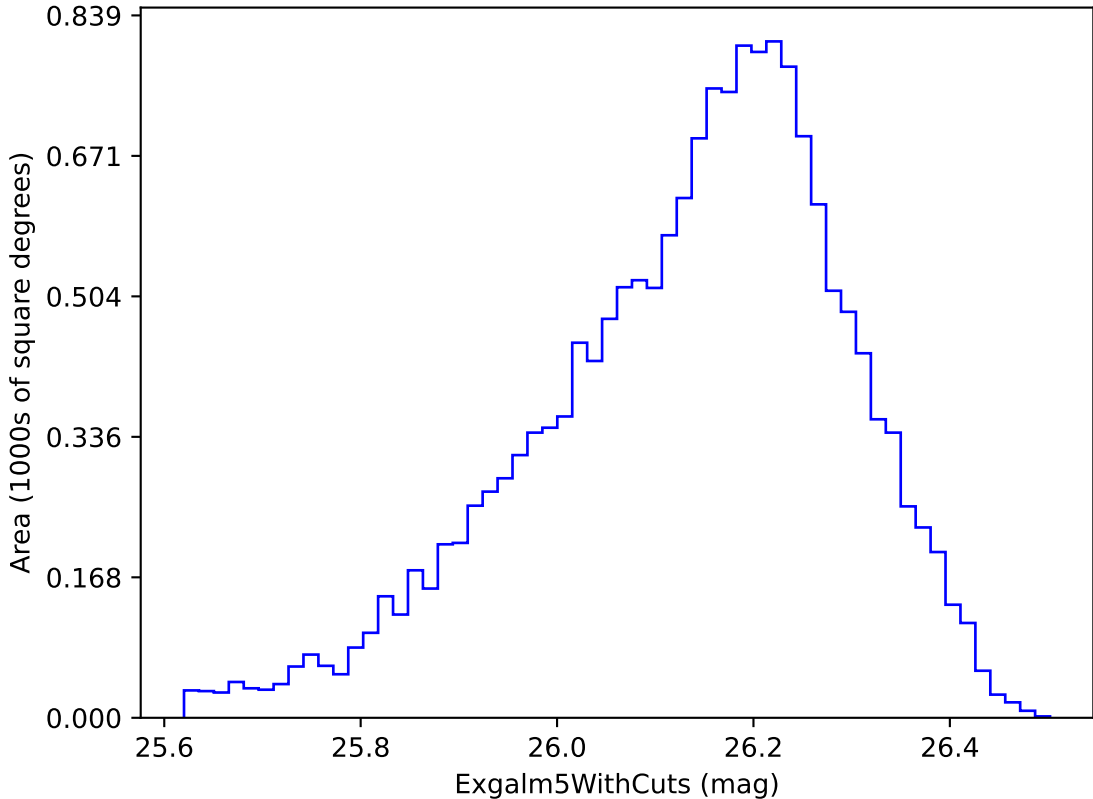
reweight_bulge_v3.3_10yrs i band non-DD year 6: ExgalM5WithCuts
