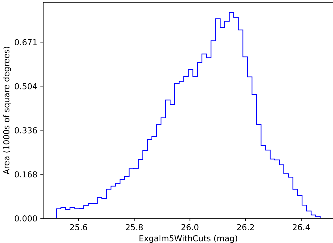
reweight_bulge_v3.3_10yrs i band non-DD year 5: ExgalM5WithCuts
