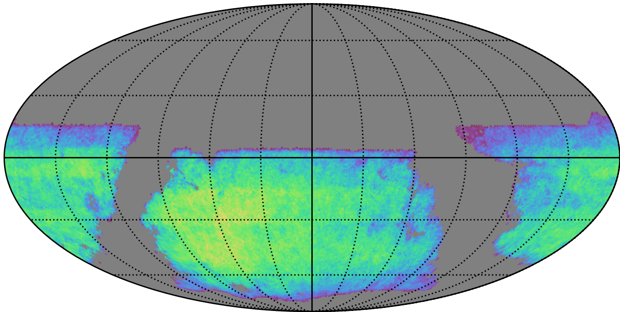
reweight_bulge_v3.3_10yrs i band non-DD year 4: ExgalM5WithCuts
