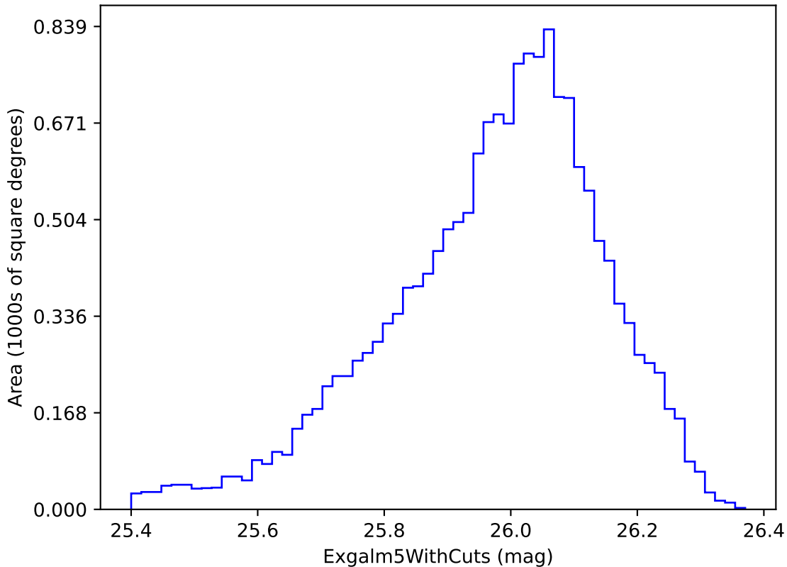
reweight_bulge_v3.3_10yrs i band non-DD year 4: ExgalM5WithCuts
