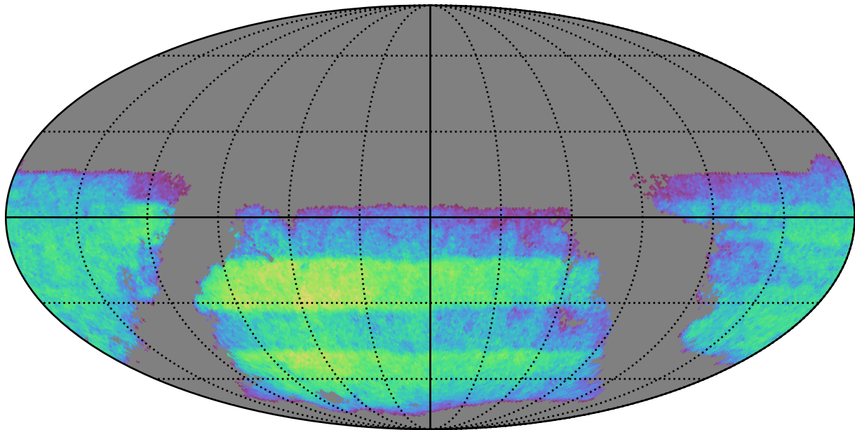
reweight_bulge_v3.3_10yrs i band non-DD year 3: ExgalM5WithCuts
