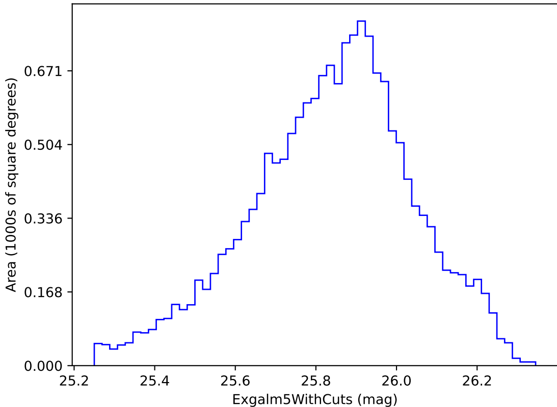
reweight_bulge_v3.3_10yrs i band non-DD year 3: Exgalml5WithCuts
