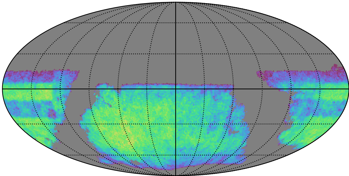
reweight_bulge_v3.3_10yrs i band non-DD year 2: ExgalM5WithCuts
