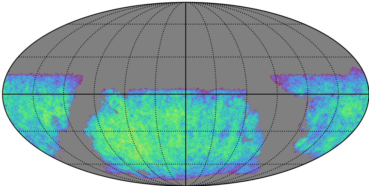
reweight_bulge_v3.3_10yrs i band non-DD year 1: ExgalM5WithCuts
