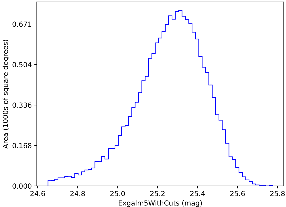
reweight_bulge_v3.3_10yrs i band non-DD year 1: ExgalM5WithCuts
