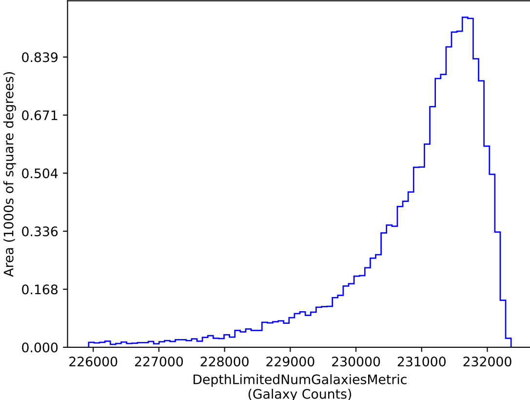
reweight_bulge_v3.3_10yrs i band galaxies non-DD: DepthLimitedNumGalaxiesMetric
