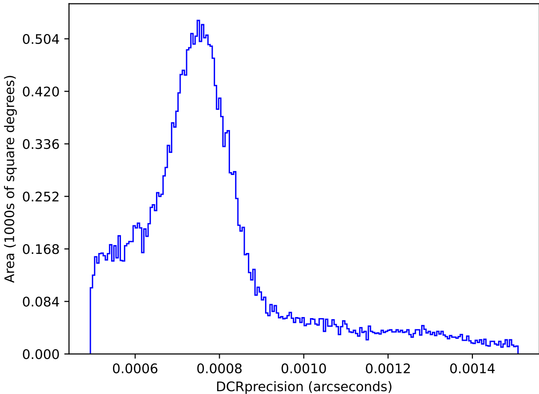
reweight_bulge_v3.3_10yrs : DCRprecision
