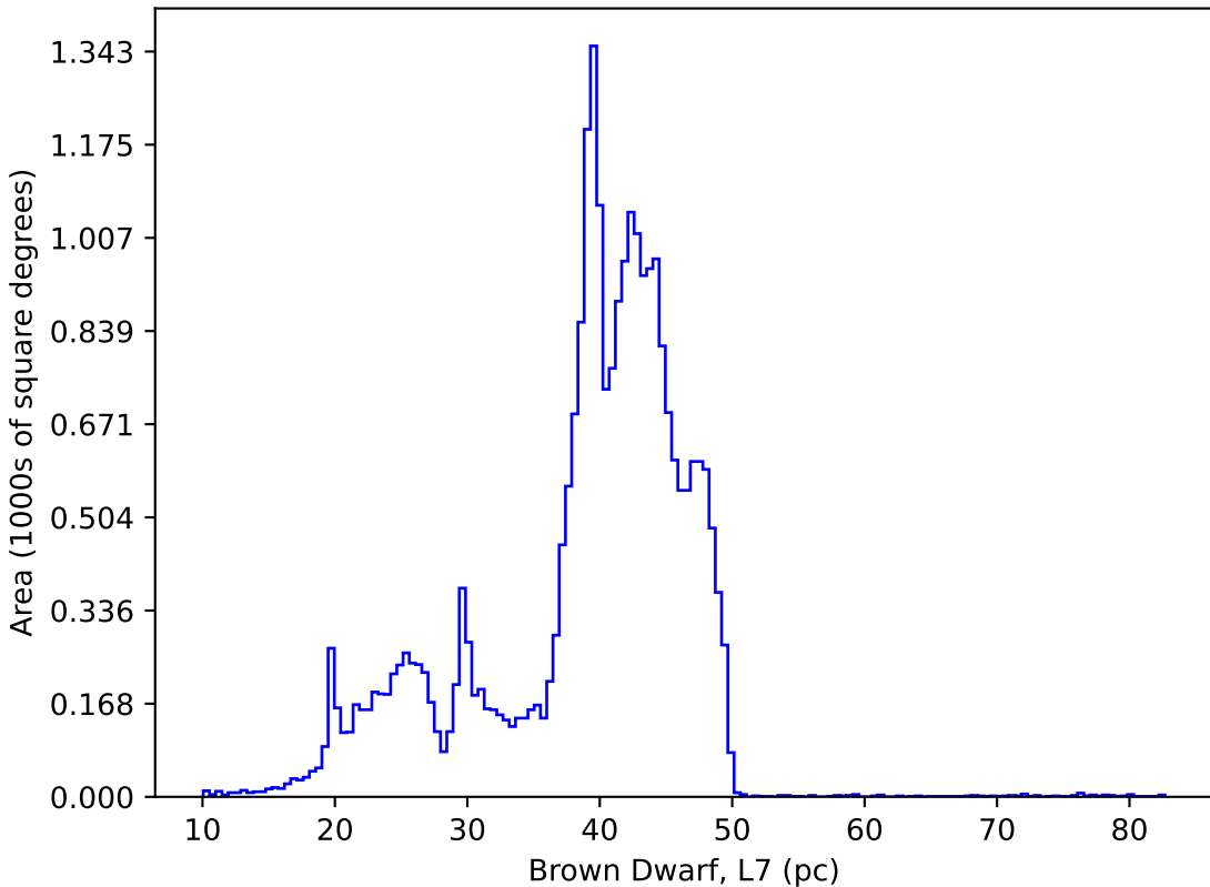
reweight_bulge_v3.3_10yrs : Brown Dwarf, L7
