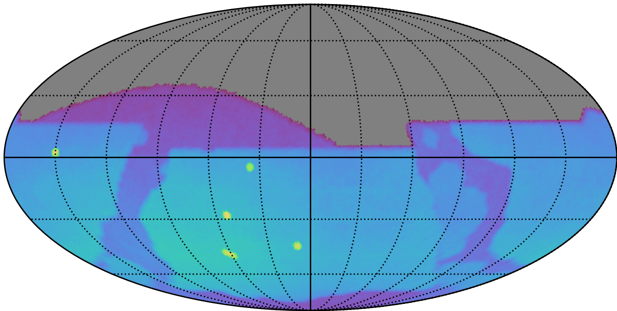
reweight_bulge_v3.3_10yrs : Brown Dwarf, L4
