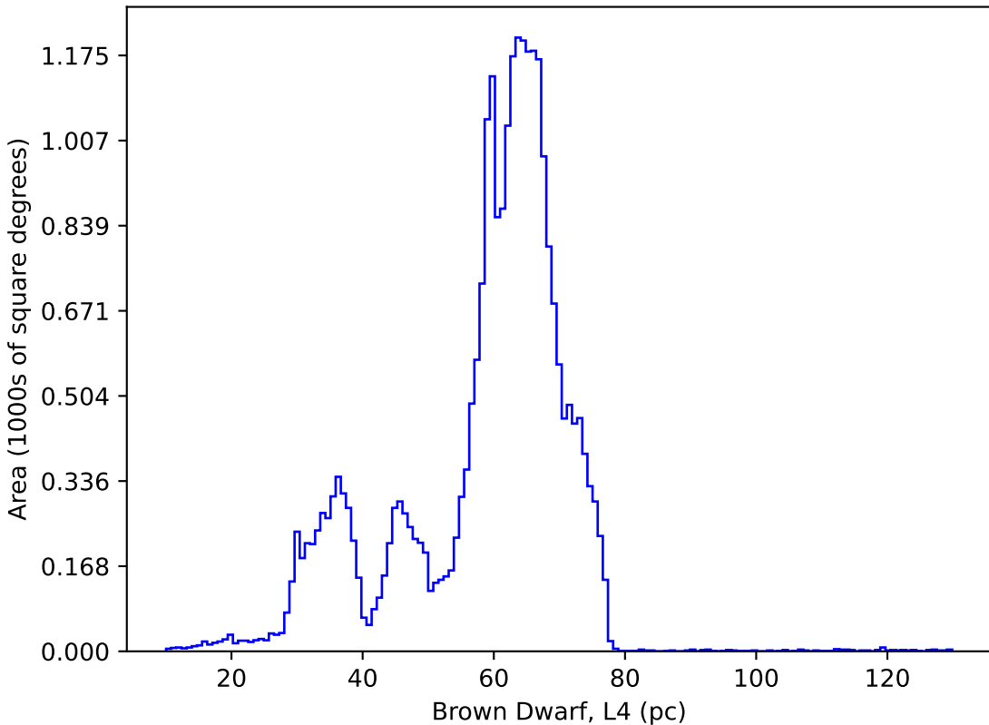
reweight_bulge_v3.3_10yrs : Brown Dwarf, L4
