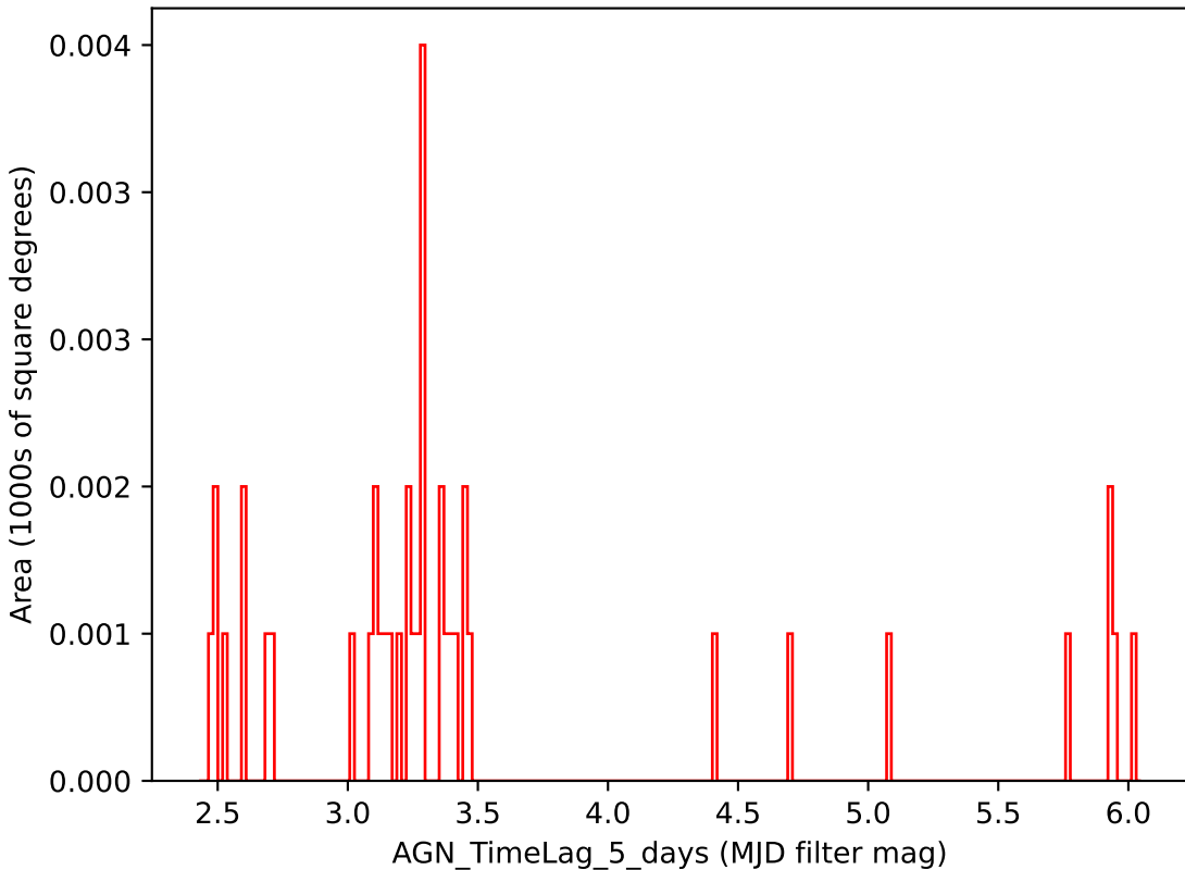
reweight_bulge_v3.3_10yrs i band: AGN_TimeLag_5_days
