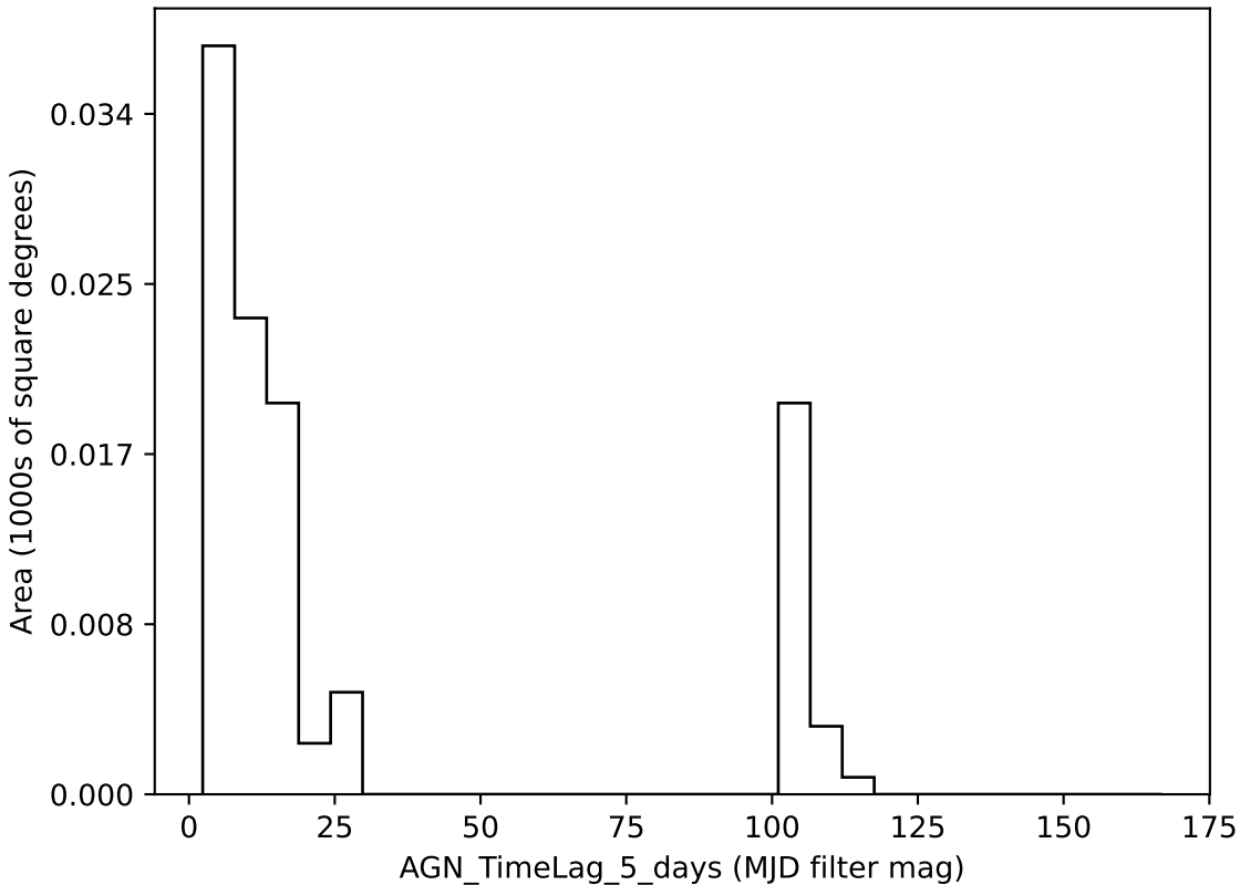
reweight_bulge_v3.3_10yrs all bands: AGN_TimeLag_5_days
