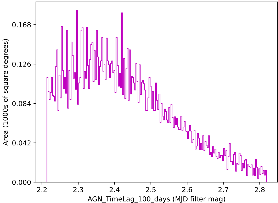
reweight_bulge_v3.3_10yrs z band: AGN_TimeLag_100_days
