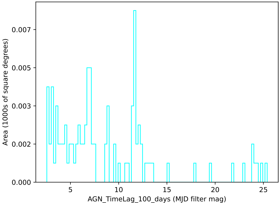
reweight_bulge_v3.3_10yrs u band: AGN_TimeLag_100_days
