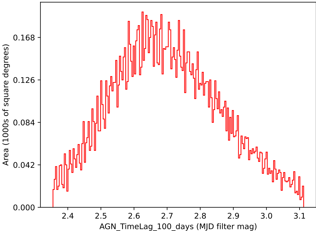
reweight_bulge_v3.3_10yrs i band: AGN_TimeLag_100_days
