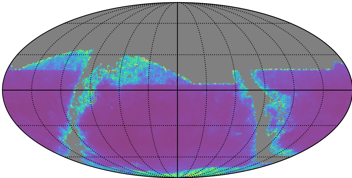
reweight_bulge_v3.3_10yrs z band: AGN SF_uncert
