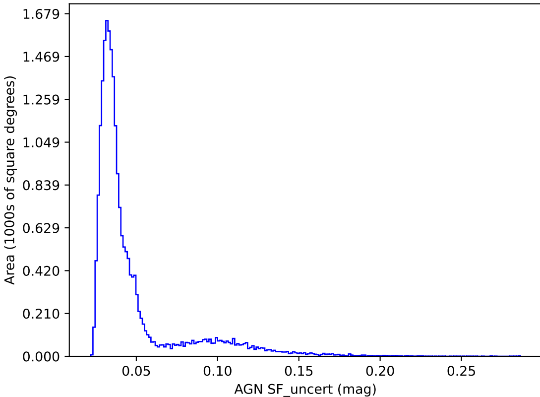
reweight_bulge_v3.3_10yrs y band: AGN SF_uncert
