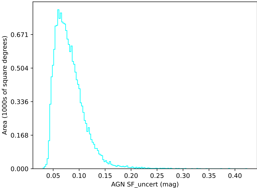
reweight_bulge_v3.3_10yrs u band: AGN SF_uncert
