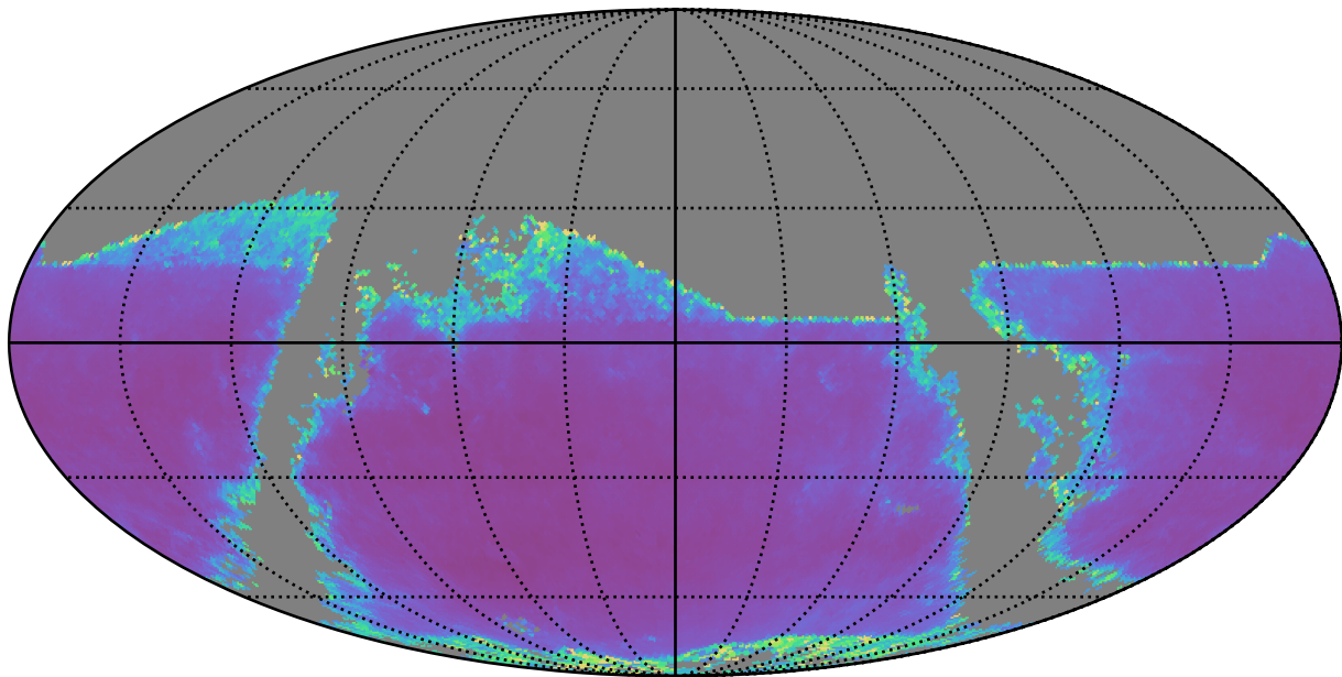
reweight_bulge_v3.3_10yrs r band: AGN SF_uncert
