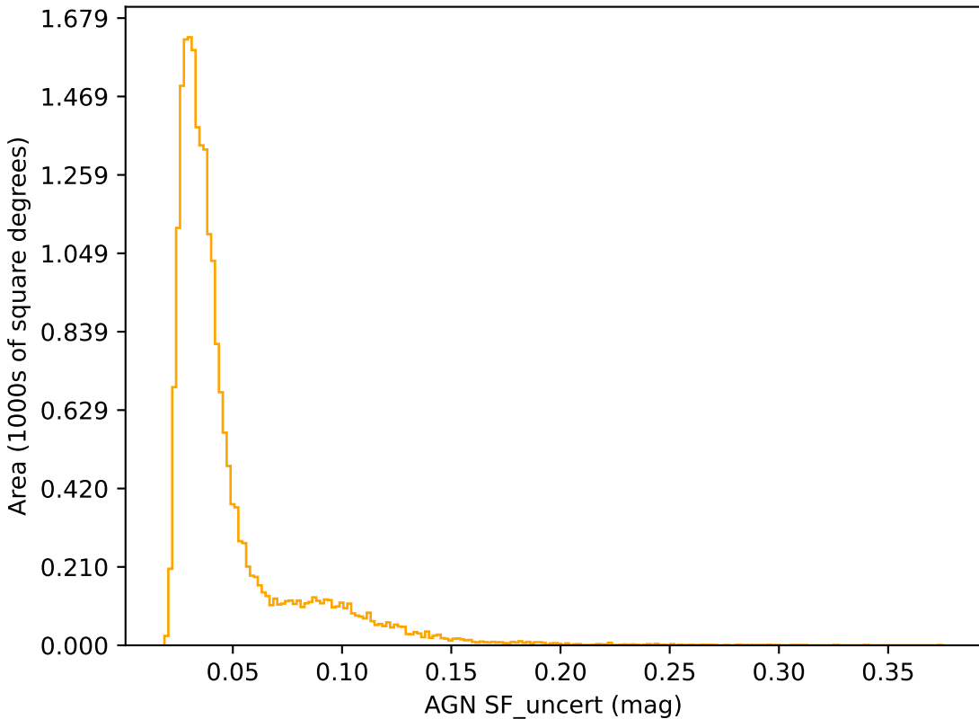
reweight_bulge_v3.3_10yrs r band: AGN SF_uncert
