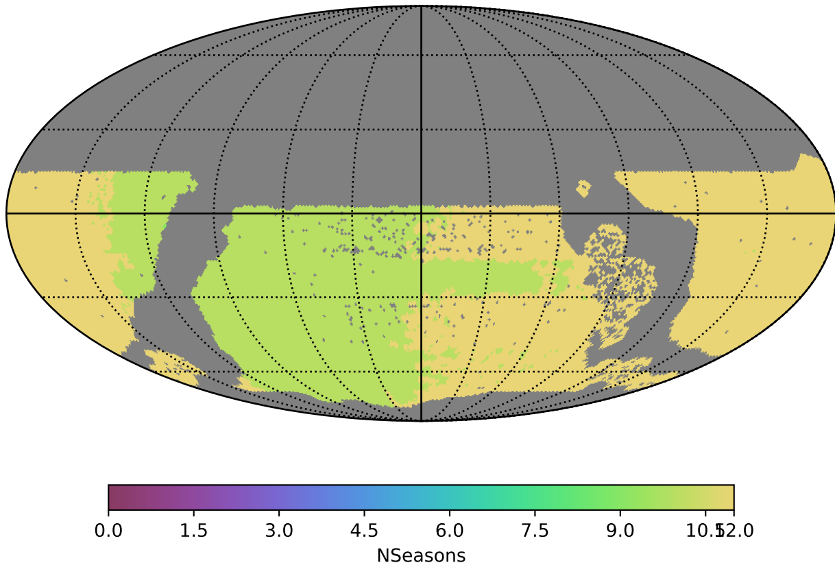
reweight_bulge_v3.3_10yrs WFD all bands: NSeasons
