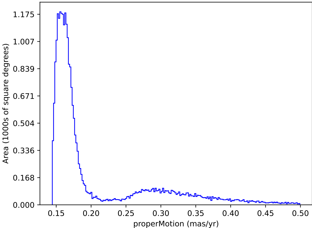
reweight_bulge_v3.3_10yrs : properMotion
