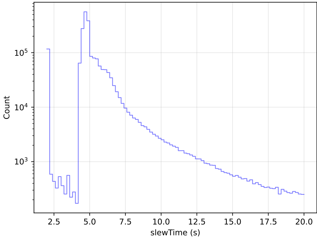
reweight_bulge_v3.3_10yrs All visits: Zoom Slew Time Histogram
