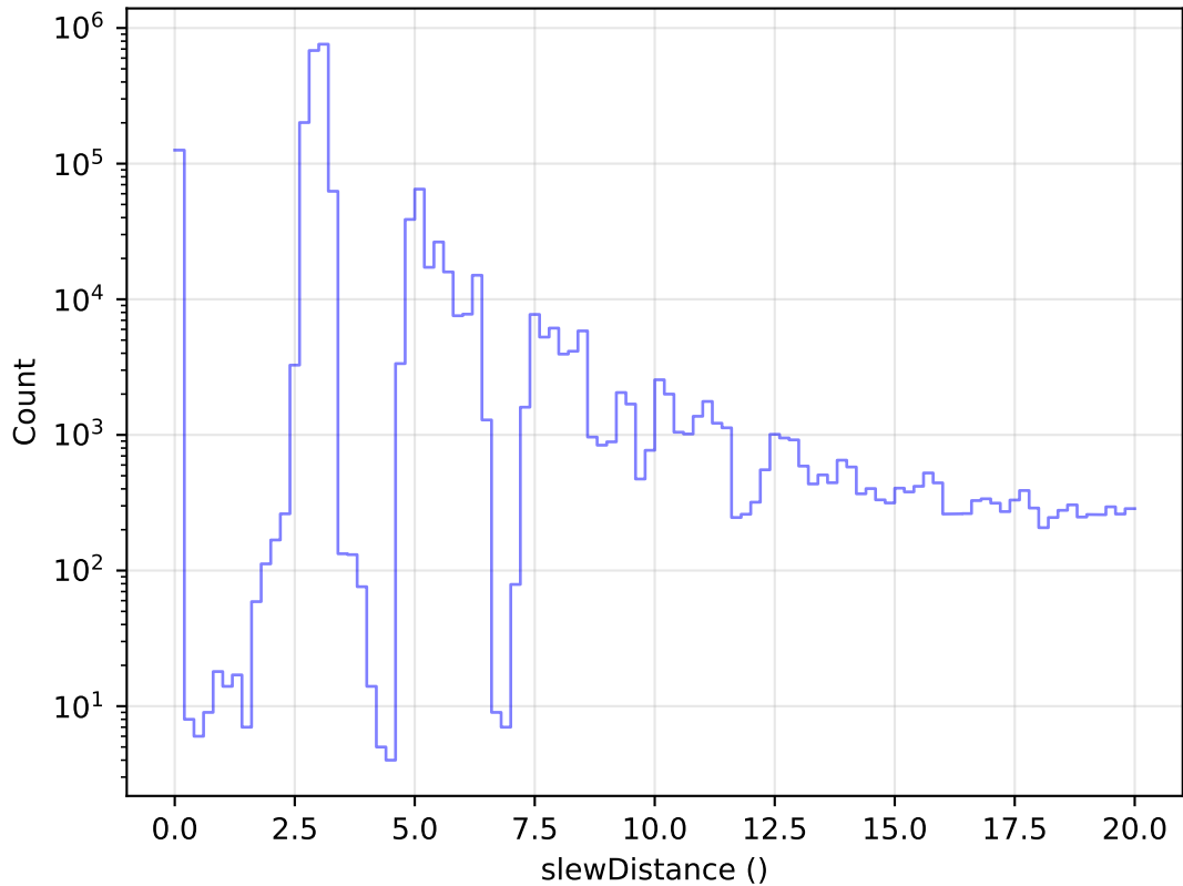
reweight_bulge_v3.3_10yrs All visits: Zoom Slew Distance Histogram
