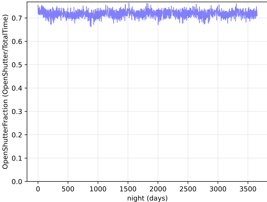
reweight_bulge_v3.3_10yrs : OpenShutterFraction
