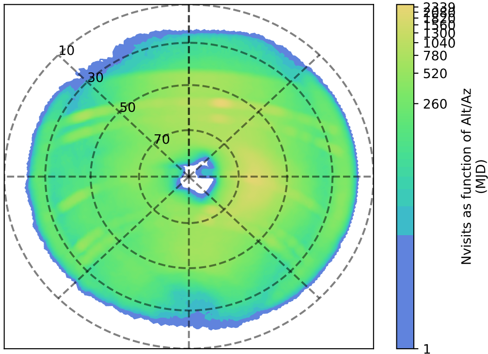
reweight_bulge_v3.3_10yrs z: Nvisits as function of Alt/Az
