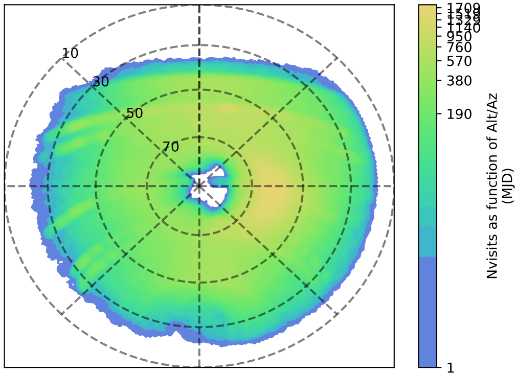
reweight_bulge_v3.3_10yrs y: Nvisits as function of Alt/Az
