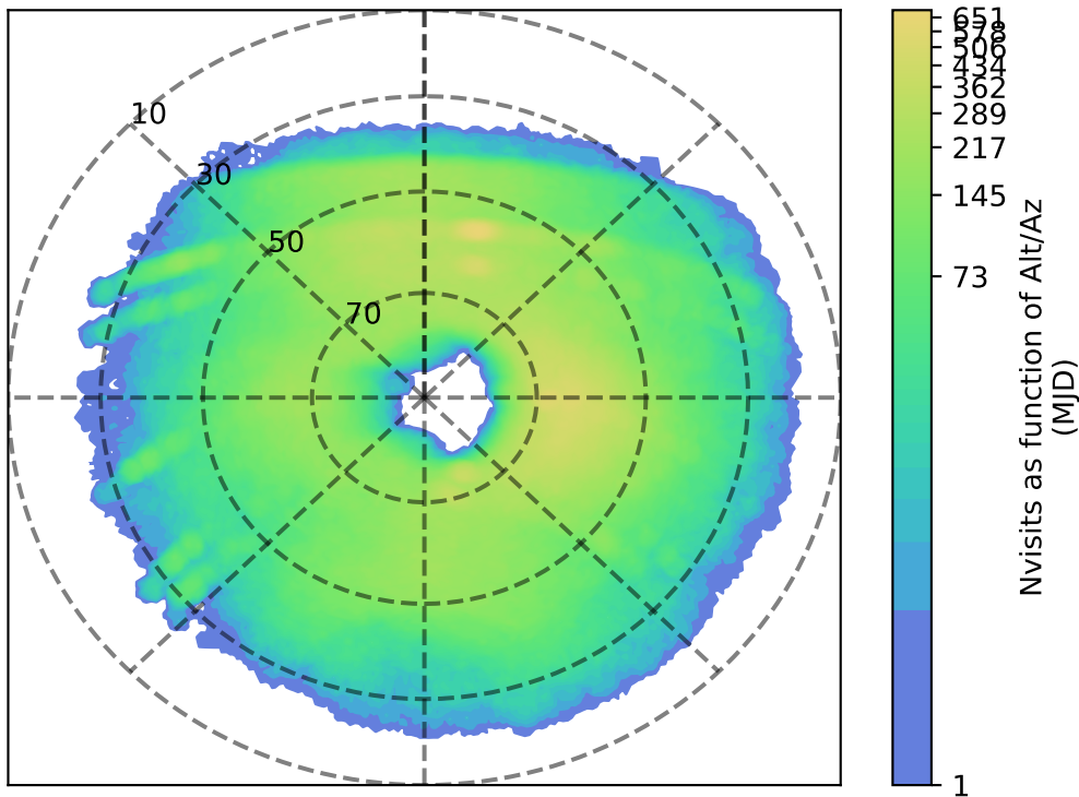
reweight_bulge_v3.3_10yrs u: Nvisits as function of Alt/Az
