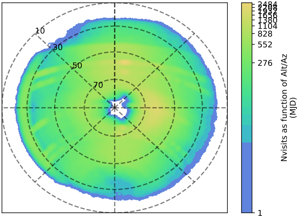
reweight_bulge_v3.3_10yrs r: Nvisits as function of Alt/Az
