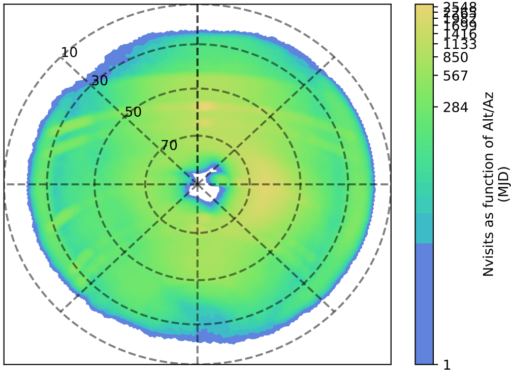
reweight_bulge_v3.3_10yrs i: Nvisits as function of Alt/Az
