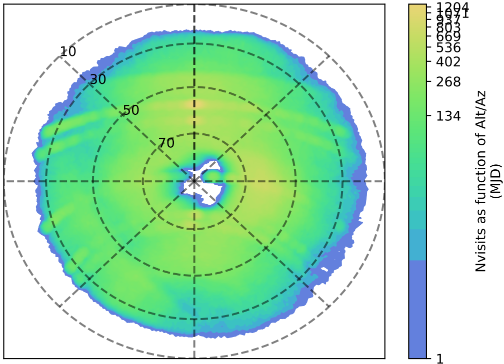
reweight_bulge_v3.3_10yrs g: Nvisits as function of Alt/Az
