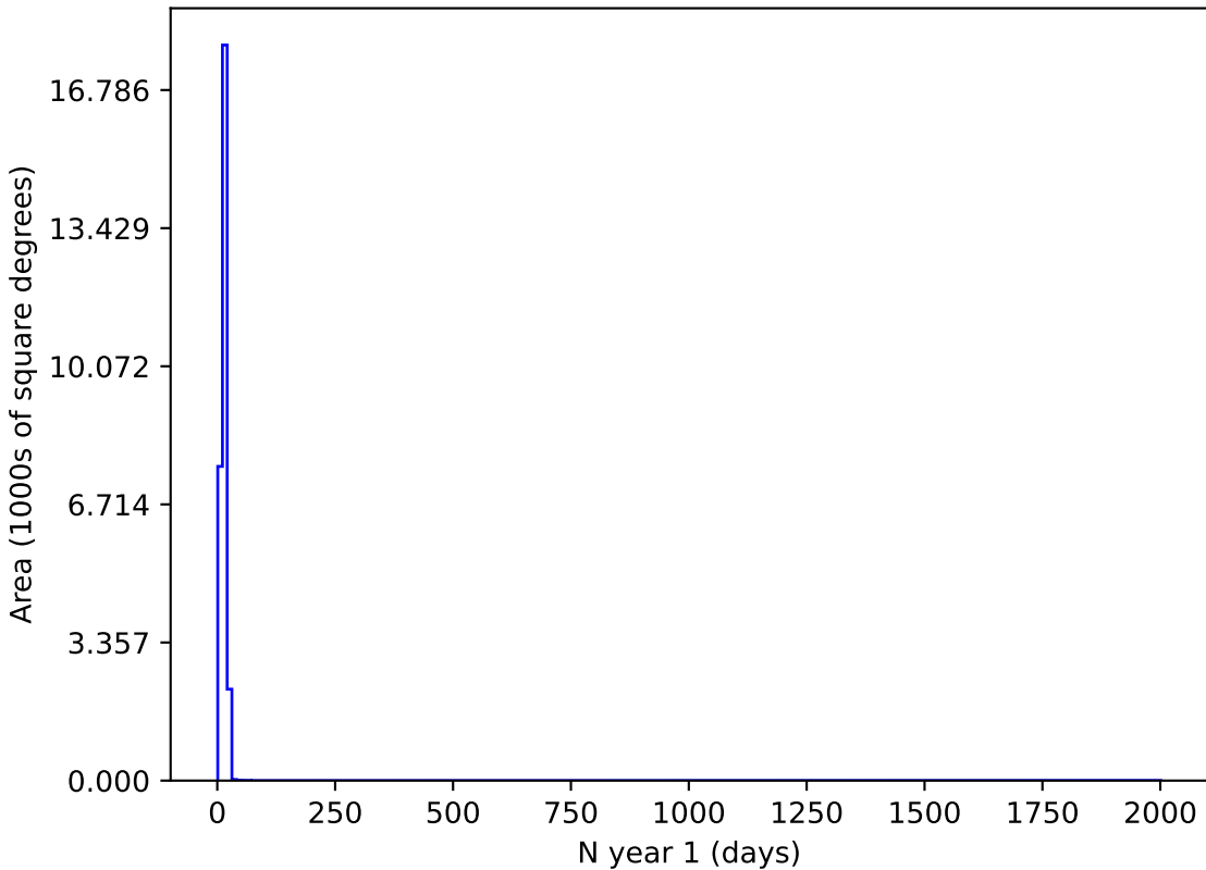
reweight_bulge_v3.3_10yrs z and night < 365: N year 1
