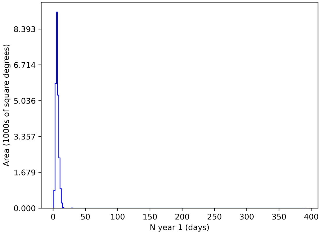
reweight_bulge_v3.3_10yrs u and night < 365: N year 1
