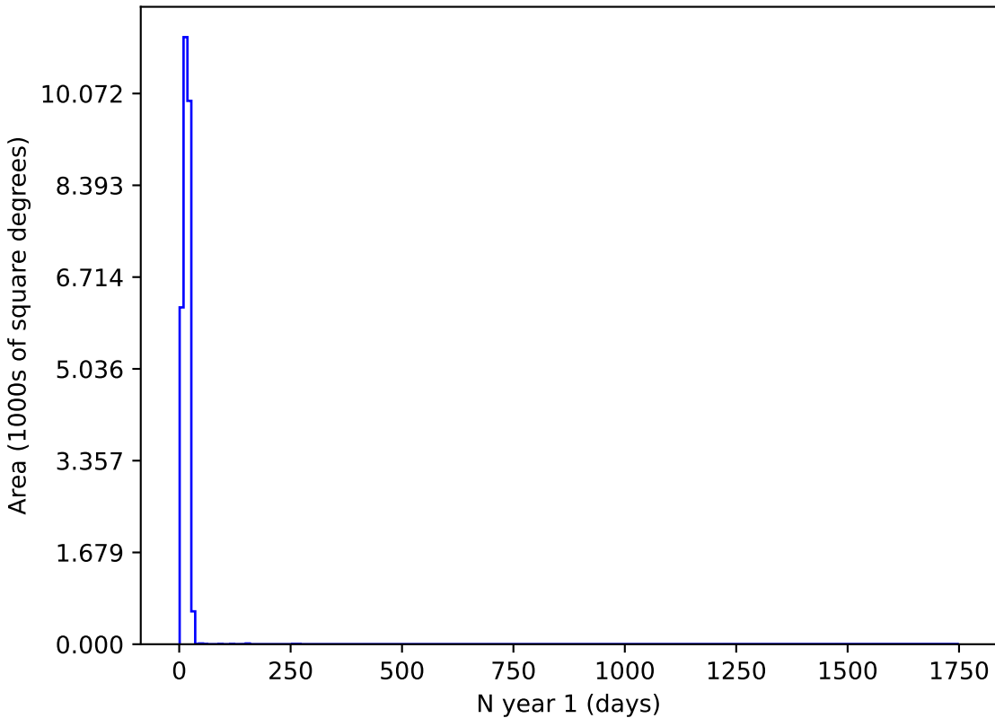
reweight_bulge_v3.3_10yrs r and night < 365: N year 1
