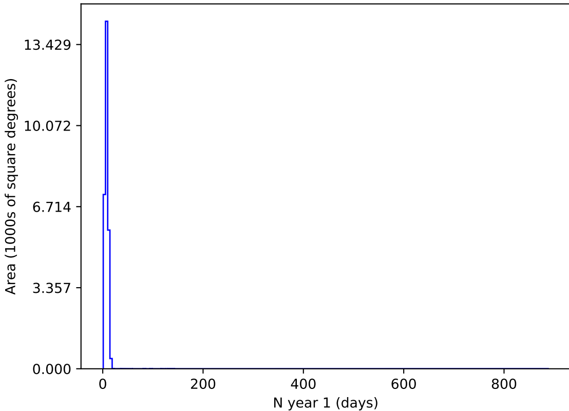
reweight_bulge_v3.3_10yrs g and night < 365: N year 1
