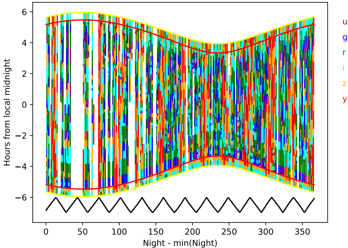
reweight_bulge_v3.3_10yrs year 8-9: Hourglass
