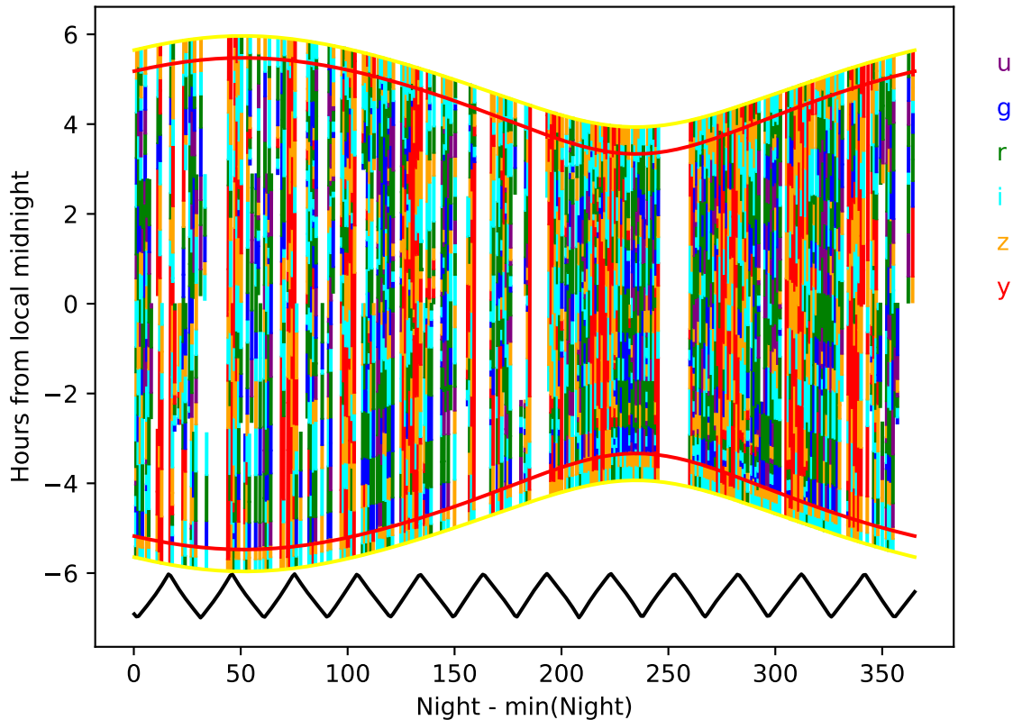
reweight_bulge_v3.3_10yrs year 5-6: Hourglass
