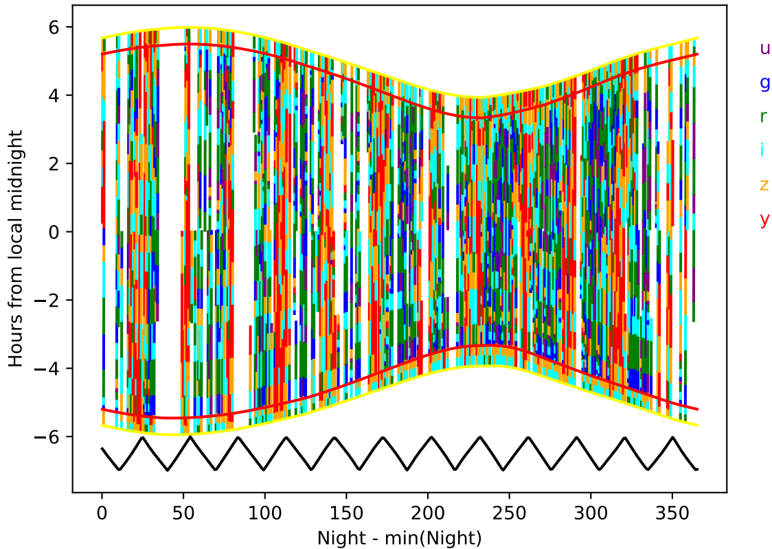
reweight_bulge_v3.3_10yrs year 4-5: Hourglass
