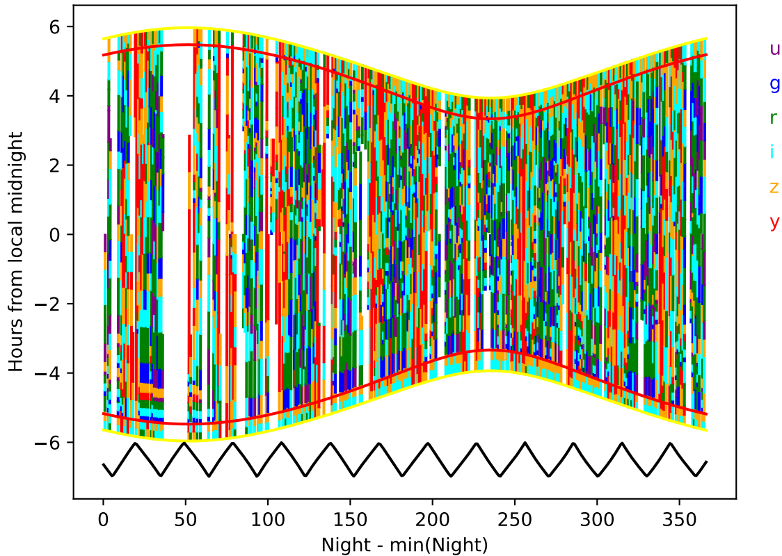
reweight_bulge_v3.3_10yrs year 2-3: Hourglass
