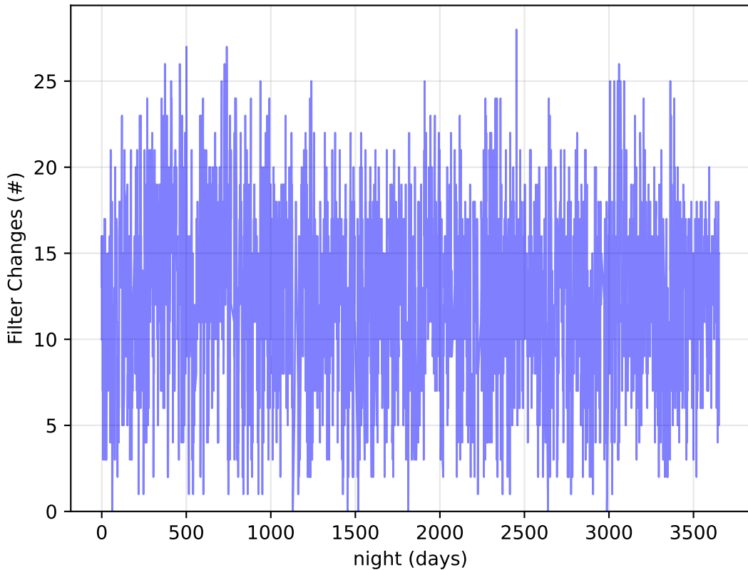
reweight_bulge_v3.3_10yrs : Filter Changes
